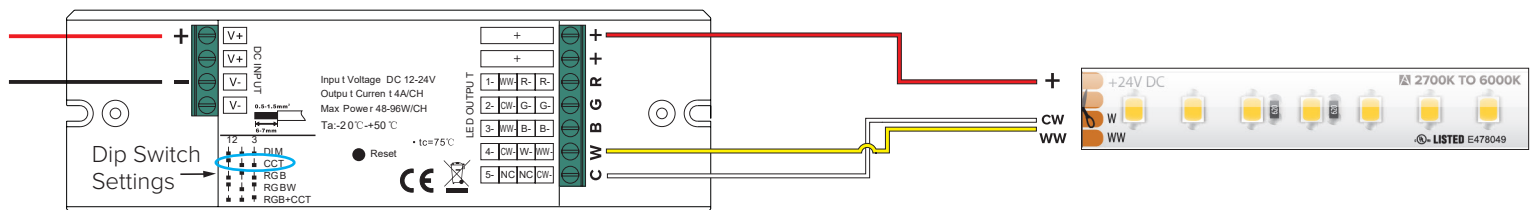
FIGURE 3 - Tunable CCT (3-Wire) Wiring Diagram
