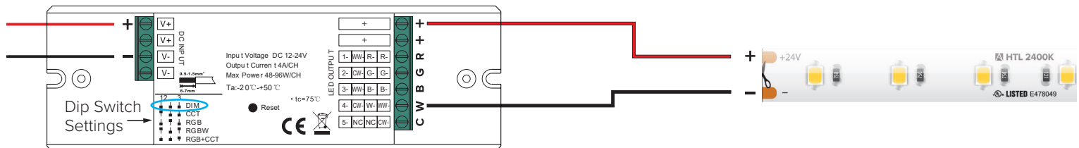
FIGURE 2 - Single Color (2-Wire) Wiring Diagram
